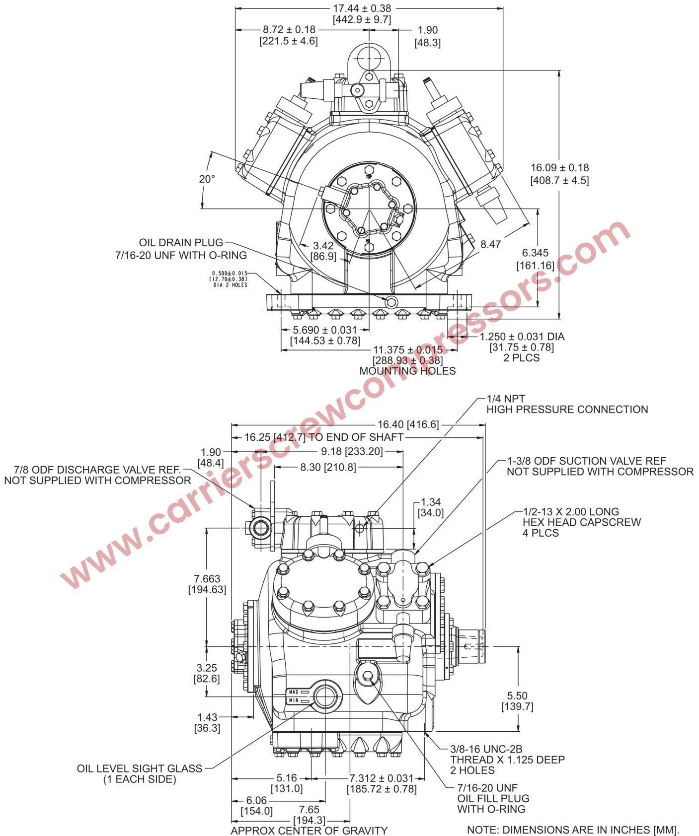
05G Compressor Components
