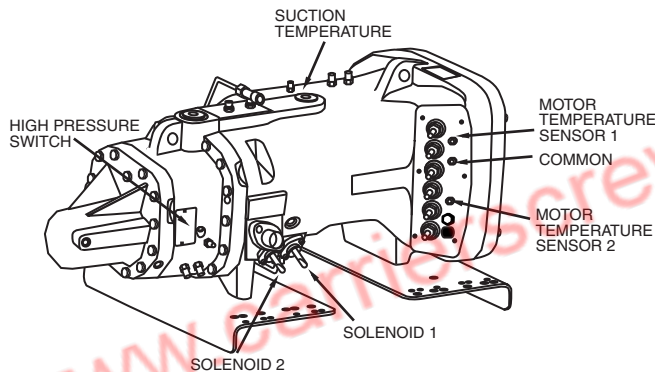
Fig. 21 — Solenoid Locations
