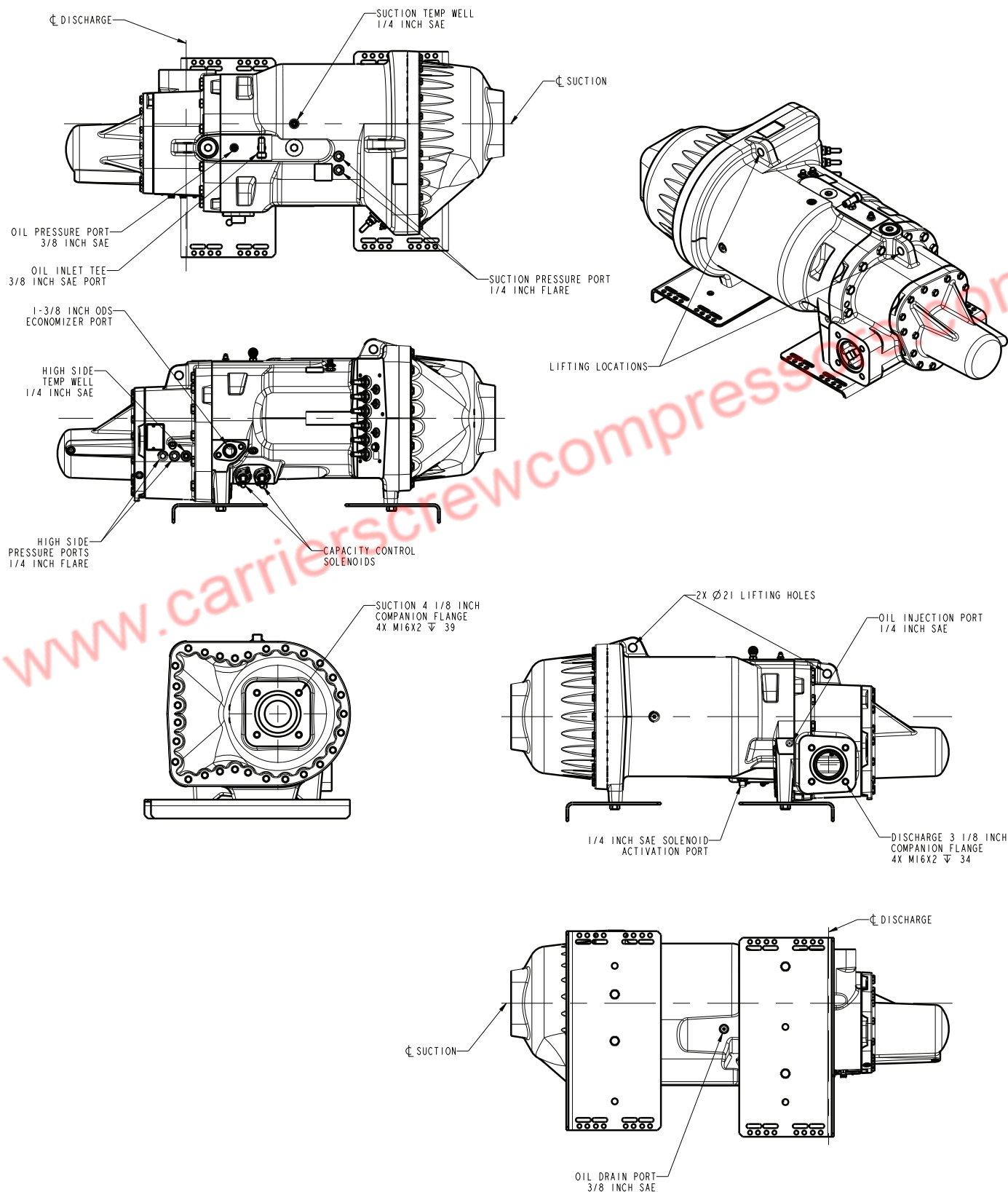
Fig. 2 — 06TT Compressor Physical Data and Connections
