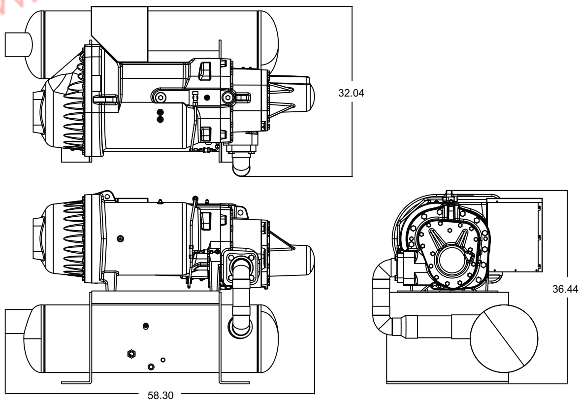
Fig. 38 — 06TTA356 Assembly Drawing
