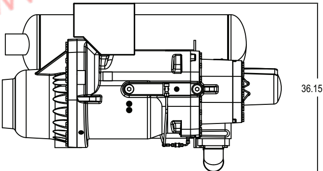
Fig. 39 — 06TUA483 Assembly Drawing
