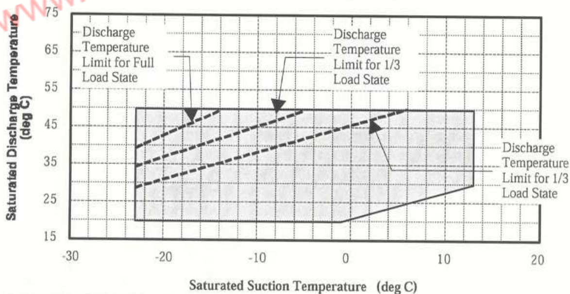
Figure 4.1-2 06NW Compressor Water-Cooled Condensing Operating Envelope
