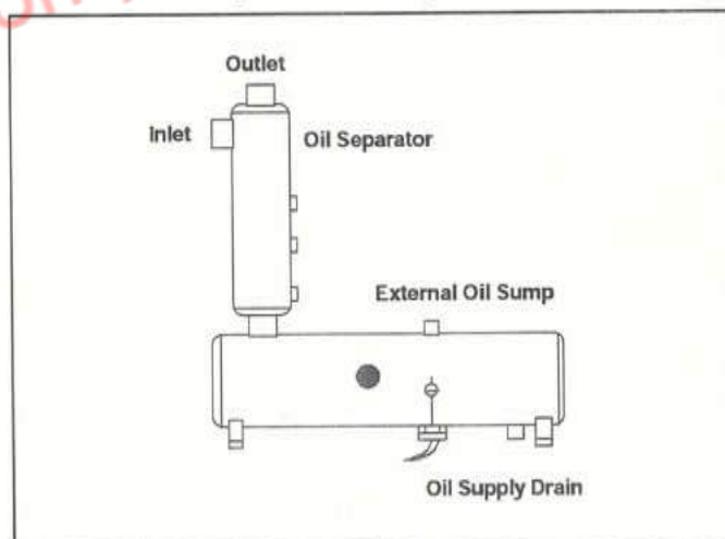
Oil Separator & Sump Schematic
